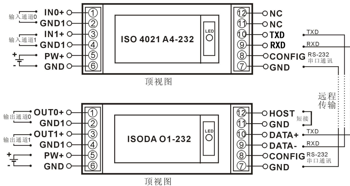
Fig.5 ISODA and ISO4021 RS-232 Communication Diagram (Top View)
