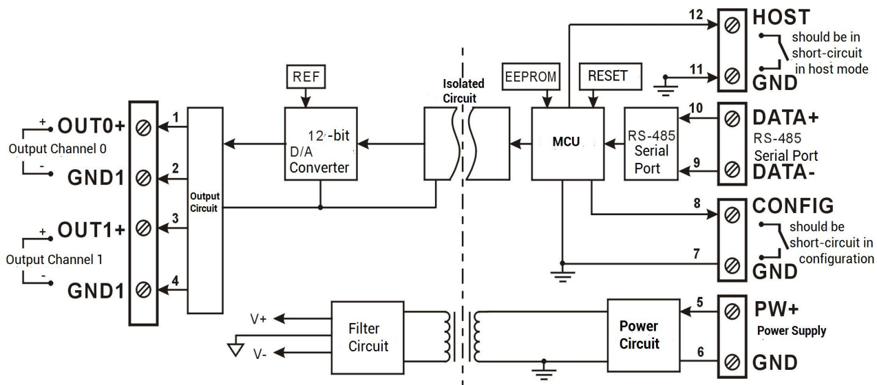
Fig. 1 ISODA functional block diagram
